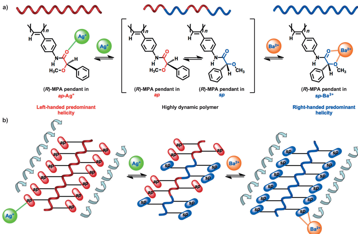
Figure 3. a) Selective modulation of the helicity induced by control of the conformation of the pendants by complexation with mono- and divalent cations (poly-1). b) Schematic representation of the amplification phenomenon indicating the ap/sp conformation of the pendants.
