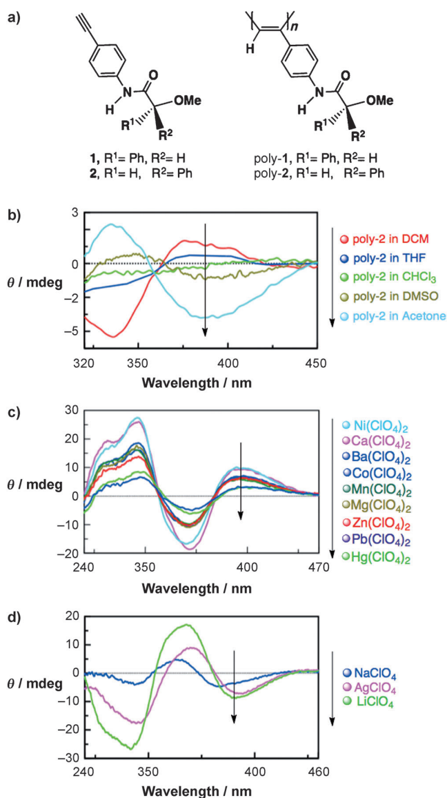
Figure 1. a) Structures of 1 , 2 , poly- 1 , and poly- 2 . b) CD spectra of poly- 2 in different solvents (0.1 mg mL -1 ). Poly- 1 generates the corresponding mirror-image spectra. c) CD spectra of poly- 1 with divalent metal cations in CHCl_3 . [14] d) CD spectra of poly- 1 with monovalent metal cations in CHCl_3 . [14]
